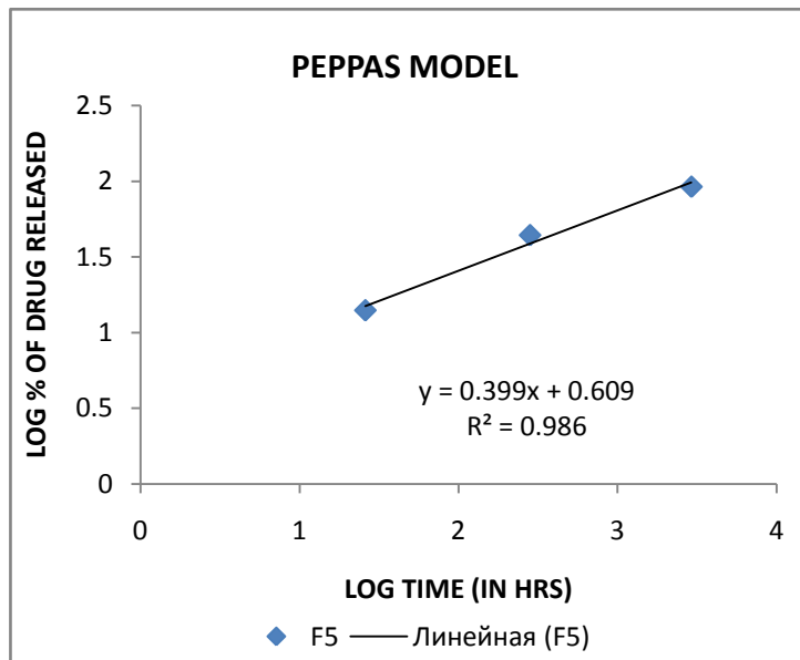
Fig 18:Peppas model
